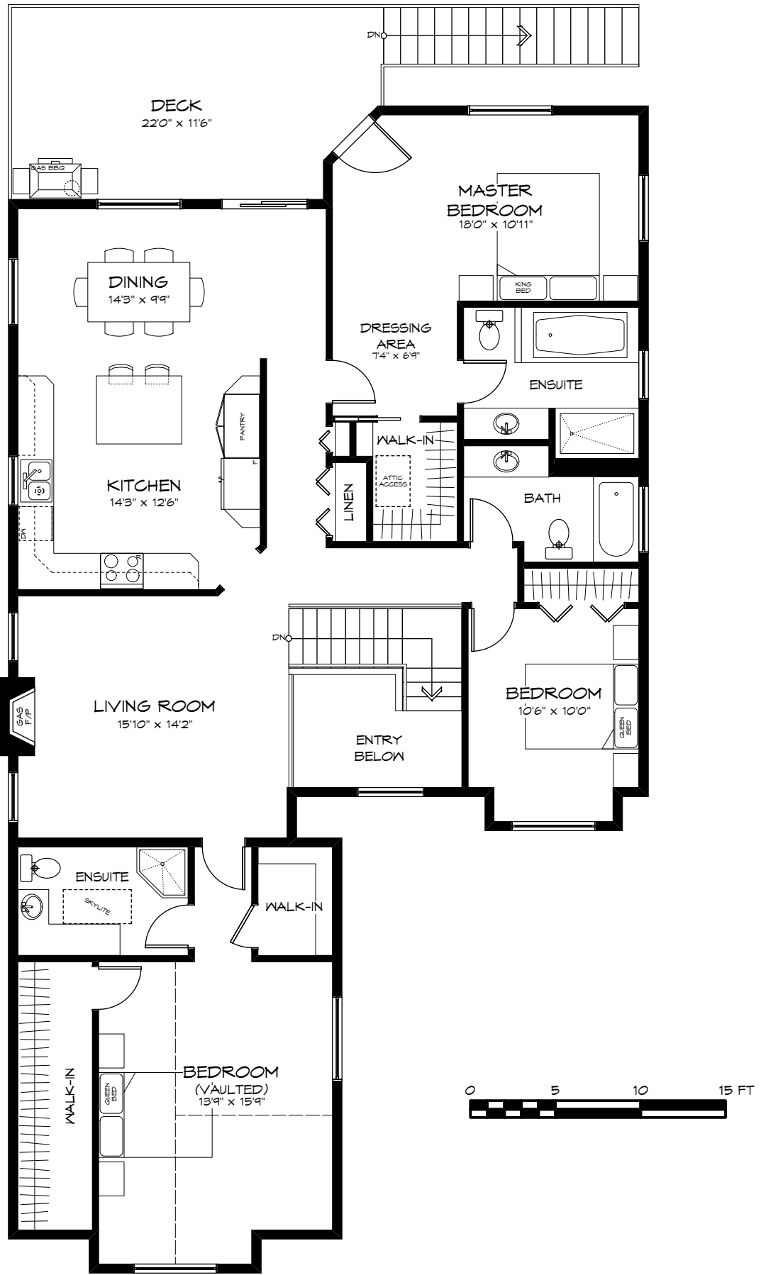
UPPER FLOOR PLAN 1835 SF
