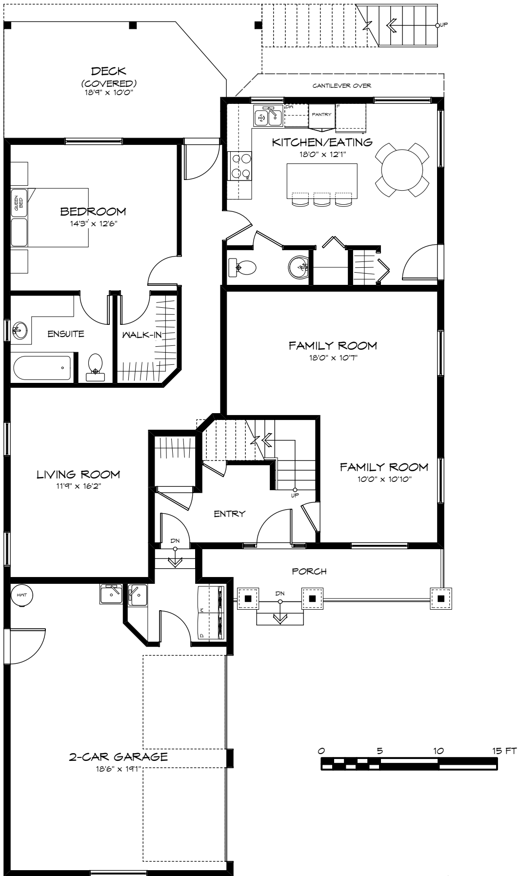
MAIN FLOOR PLAN 1480 SF (+ GARAGE)
